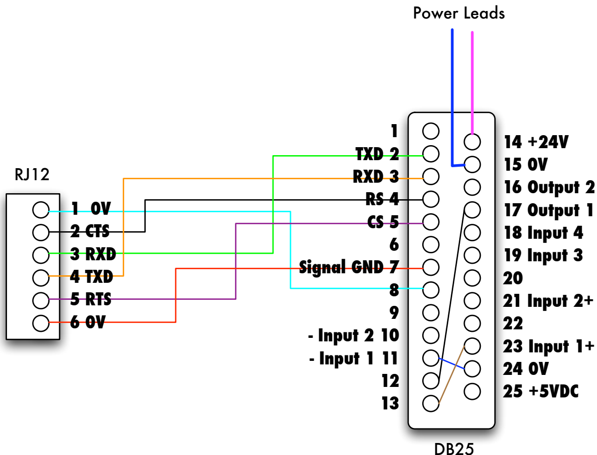
DB25 connector vs Molex 12 pin Equivalents
